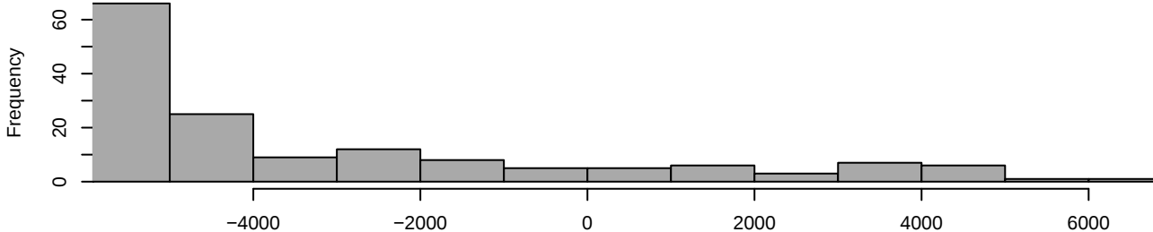
histogram
