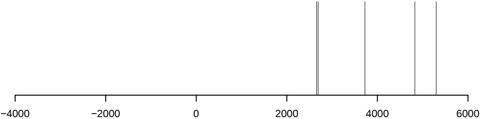
rugplot
