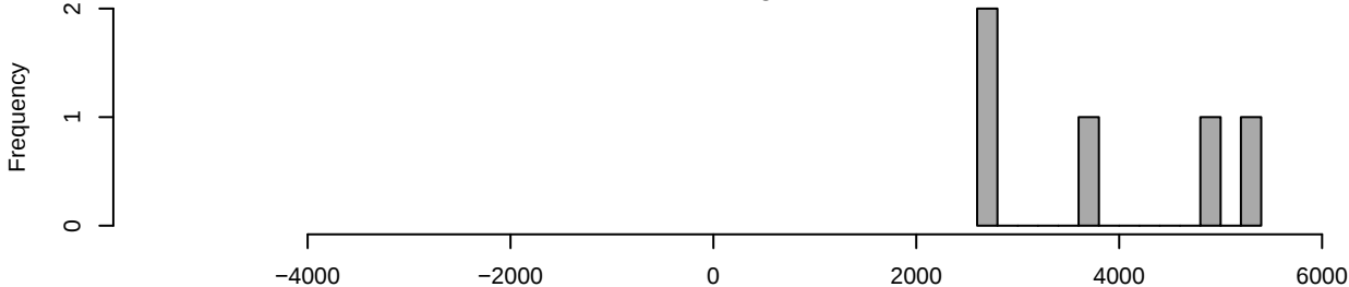
histogram
