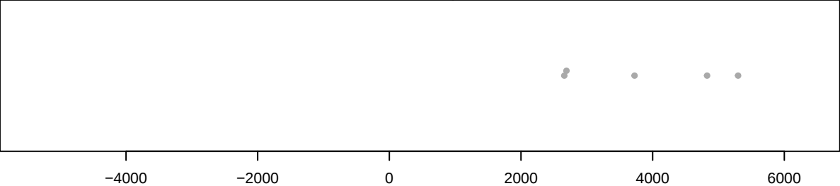
beeswarm plot
