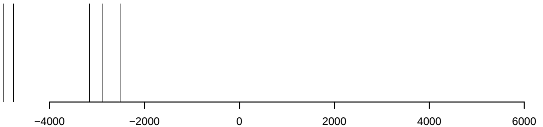
rugplot
