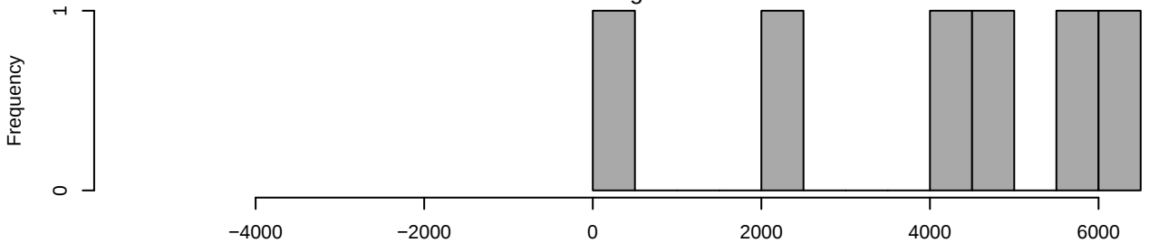
histogram
