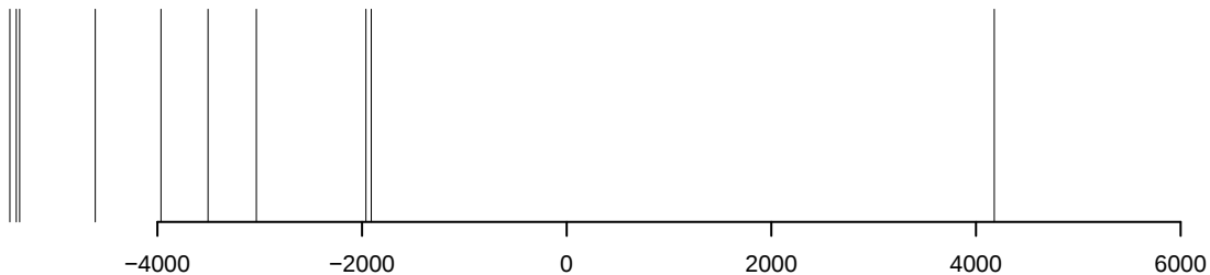
rugplot
