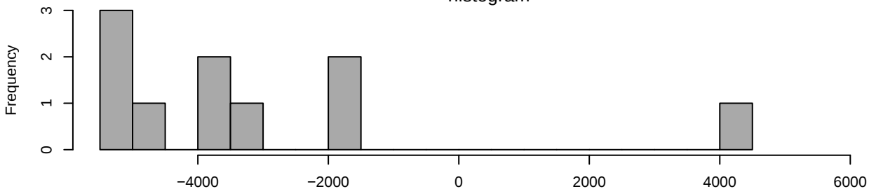
histogram
