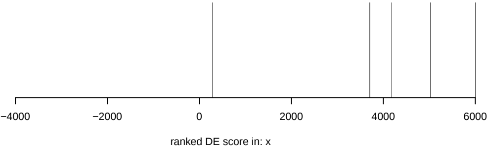
rugplot
