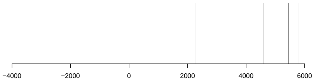
rugplot
