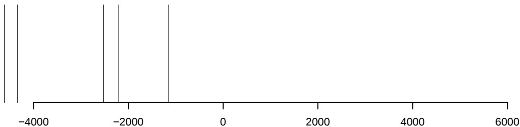
rugplot
