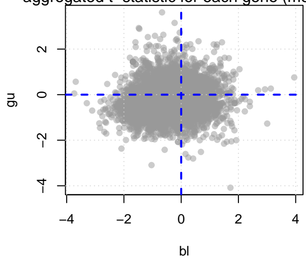
aggregated t-statistic for each gene (median)
