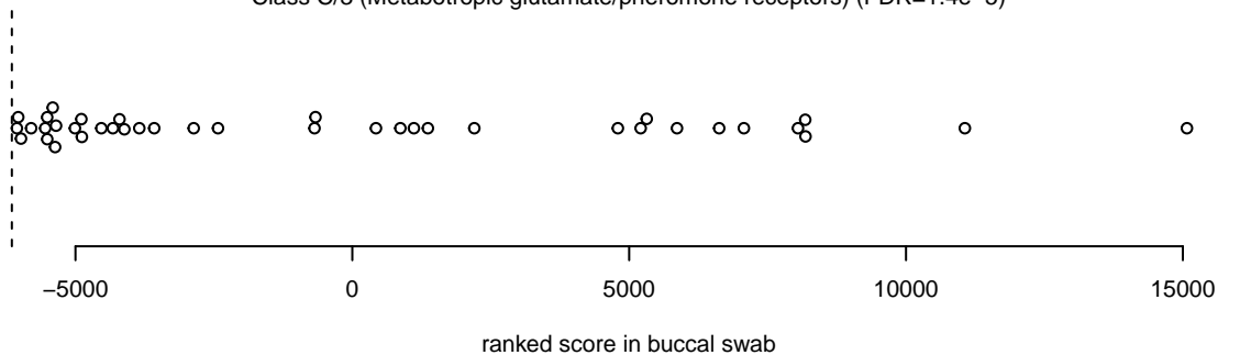
Class C/3 (Metabotropic glutamate/pheromone receptors) (FDR=1.4e-5)
