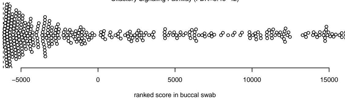
Olfactory Signaling Pathway (FDR=5.4e-42)
