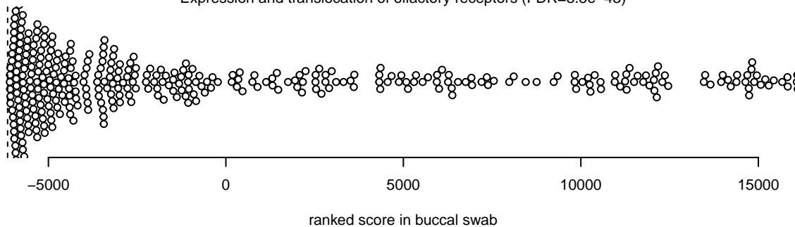
Expression and translocation of olfactory receptors (FDR=8.5e-43)
