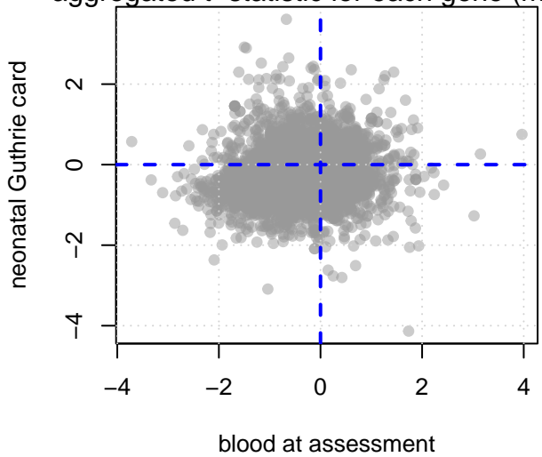
aggregated t-statistic for each gene (mean)
