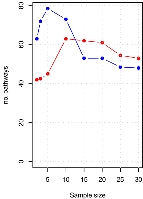
no. inconsistent pathways FDR<0.05
