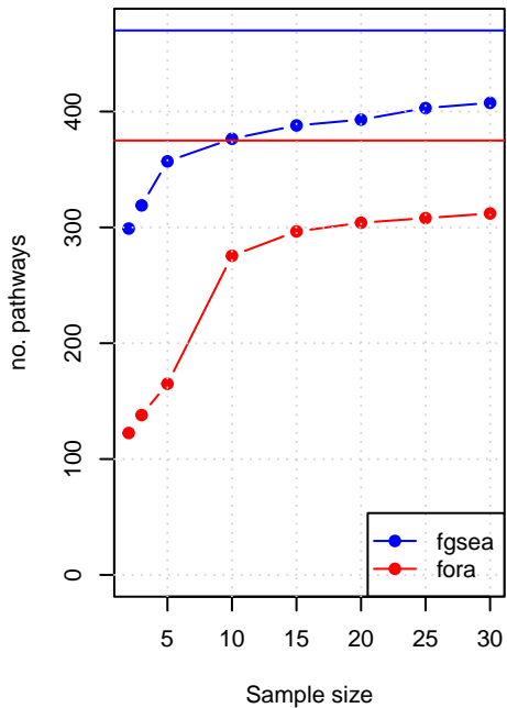
no. consistent pathways FDR<0.05
