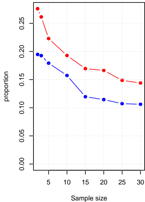
Proportion of inconsistent pathways
