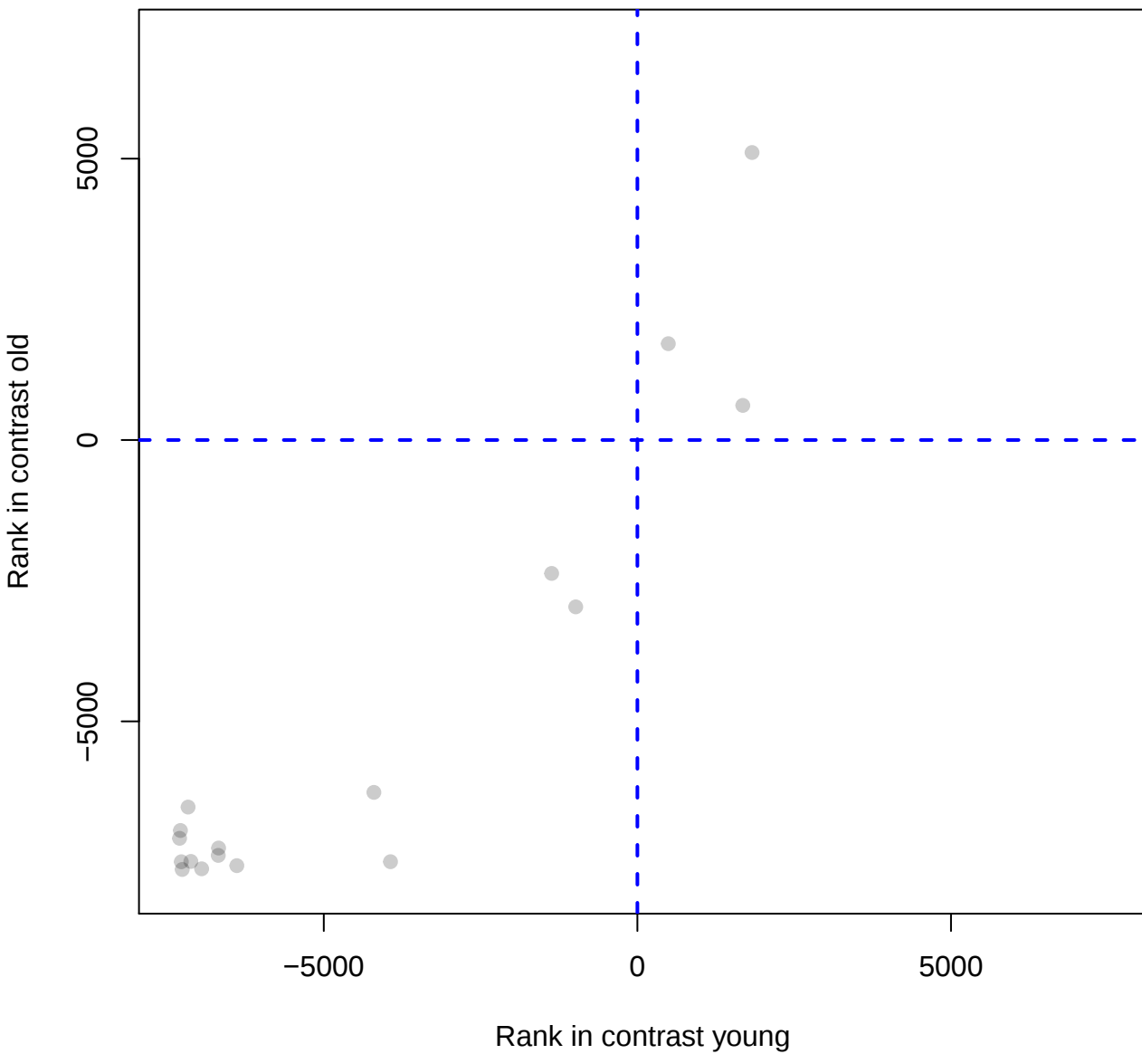
KMT2C_None_Epithelium_35684
