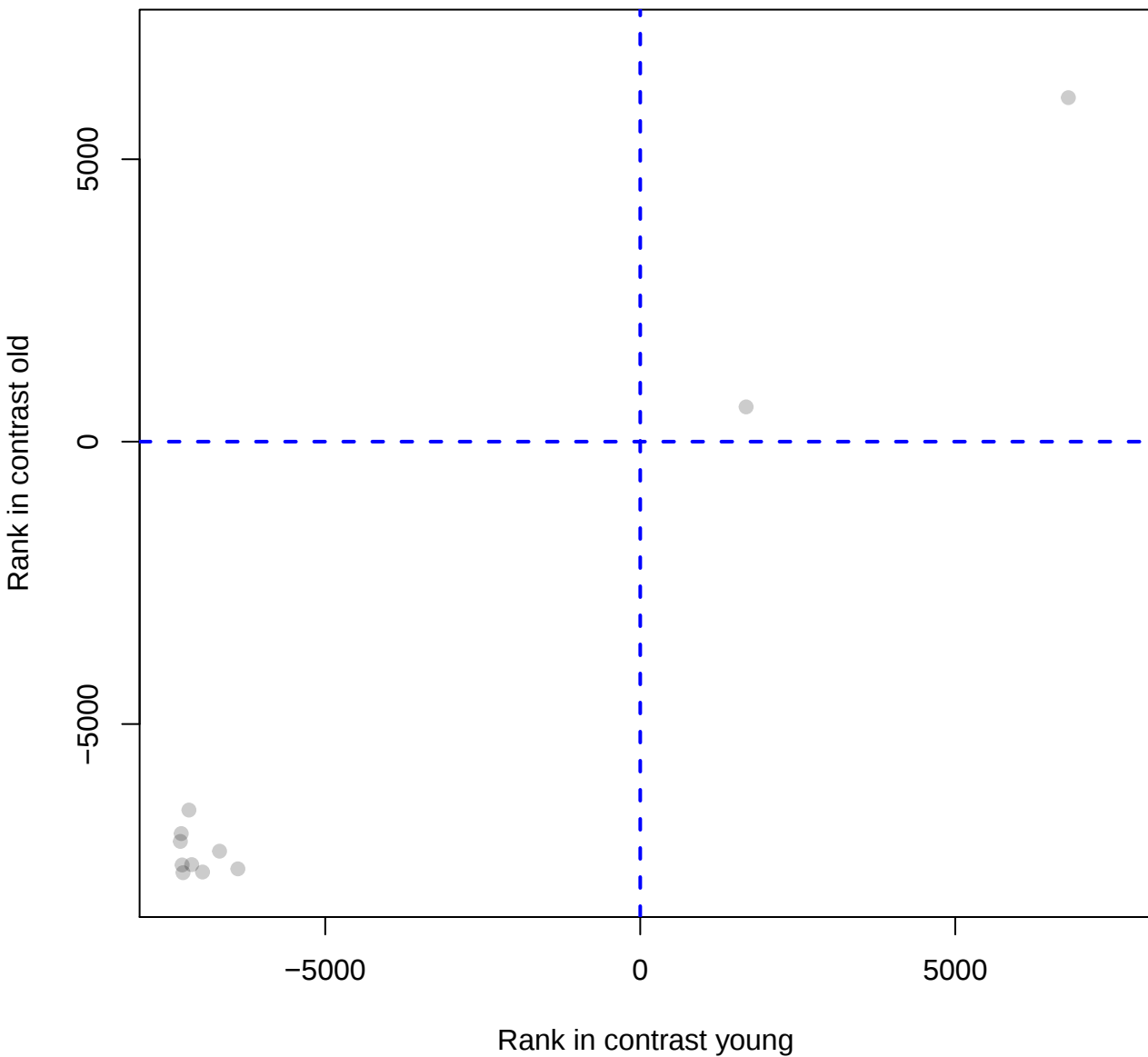
IRF4_None_TLymphocyte_53640
