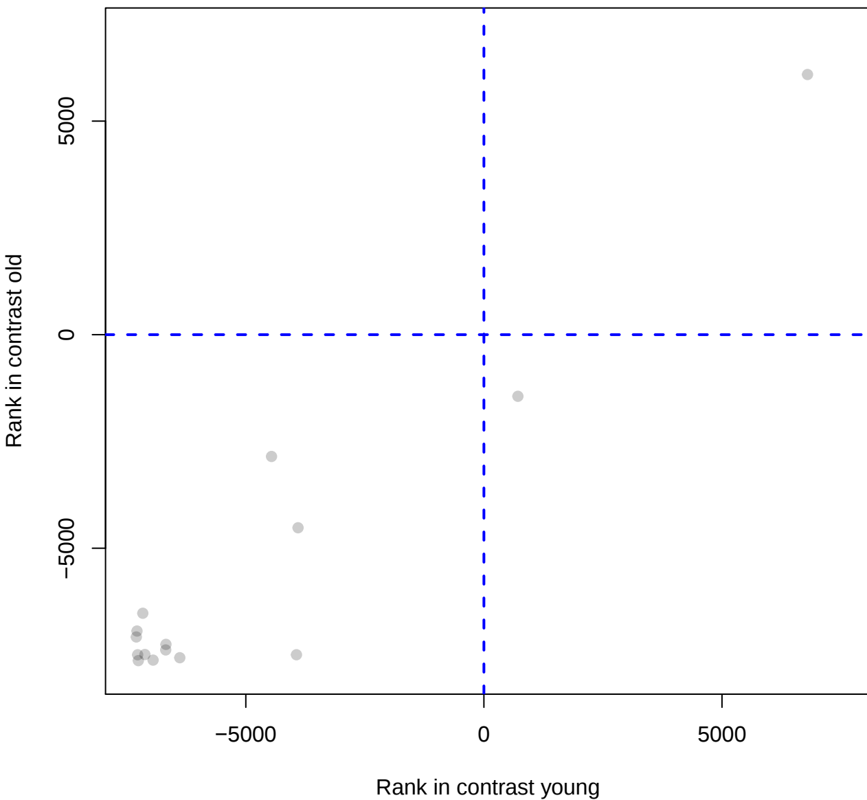
WDR5_None_NeuralProgenitorCell_41360
