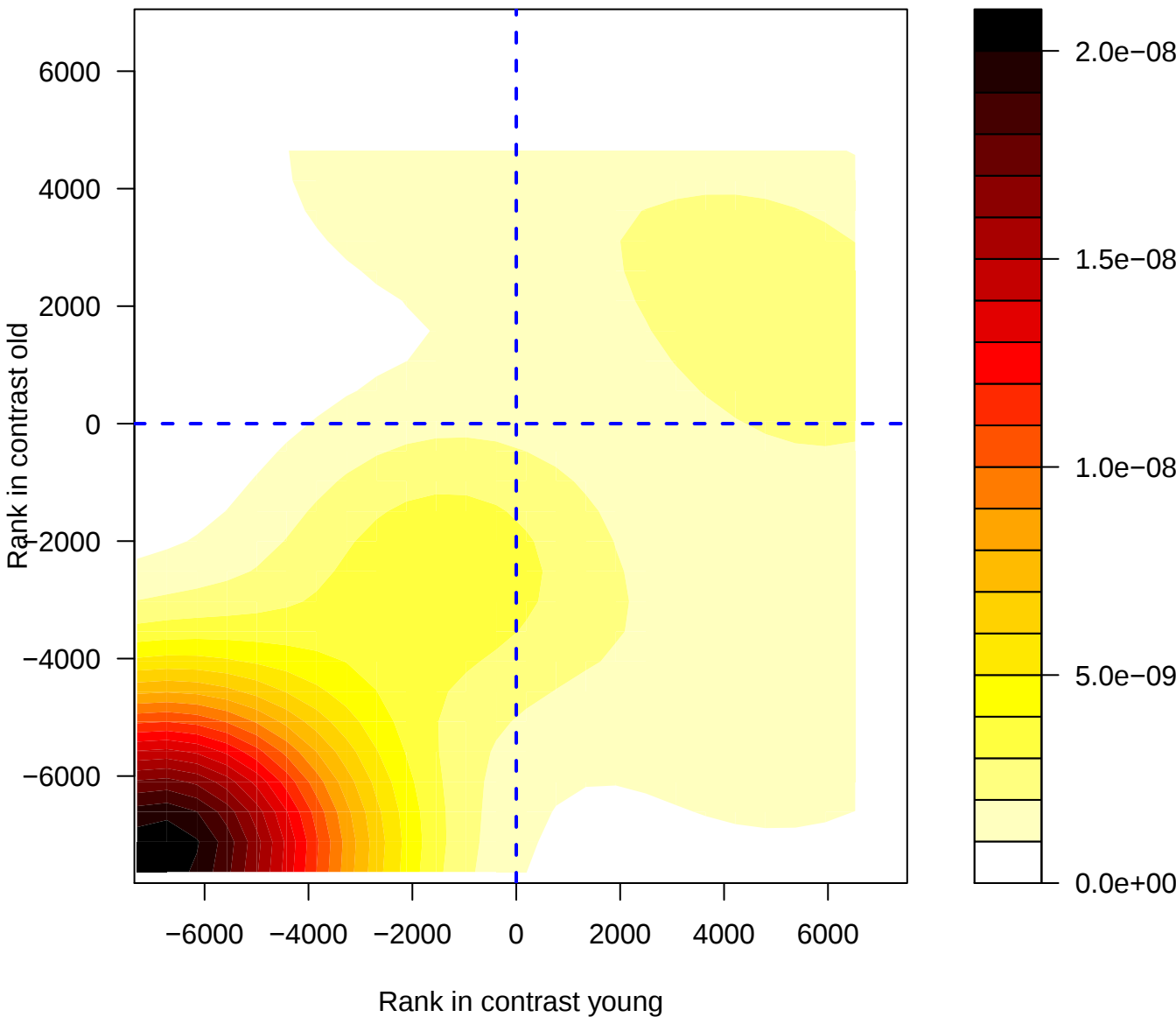
BRDU_None_BLymphocyte_32927
