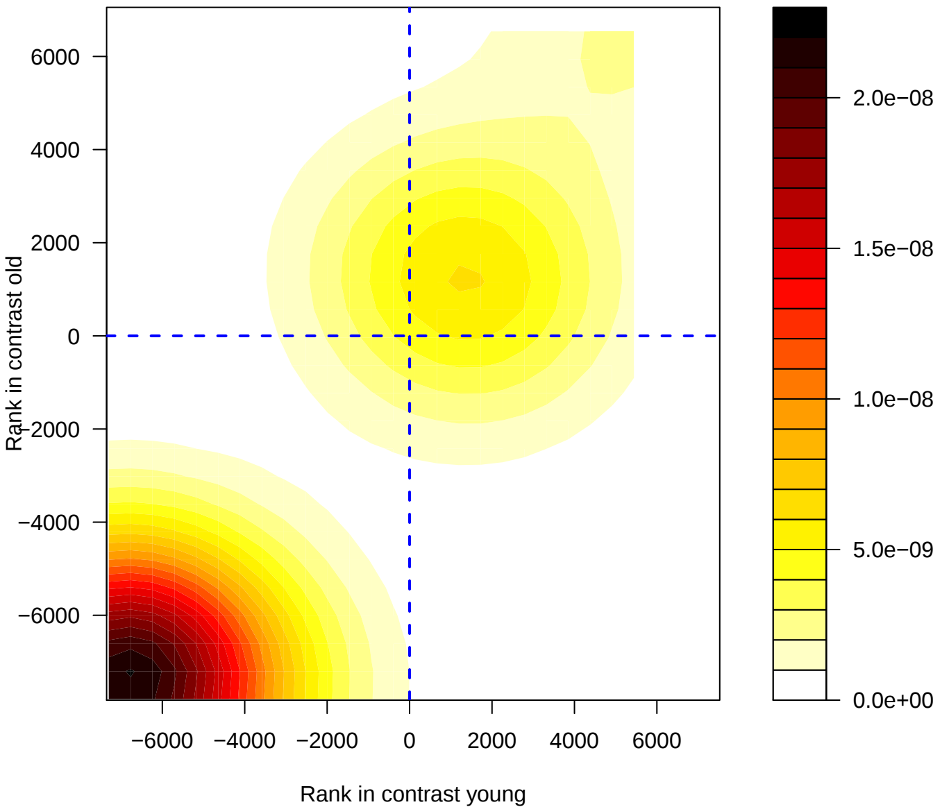
BRD2_None_Macrophage_5094
