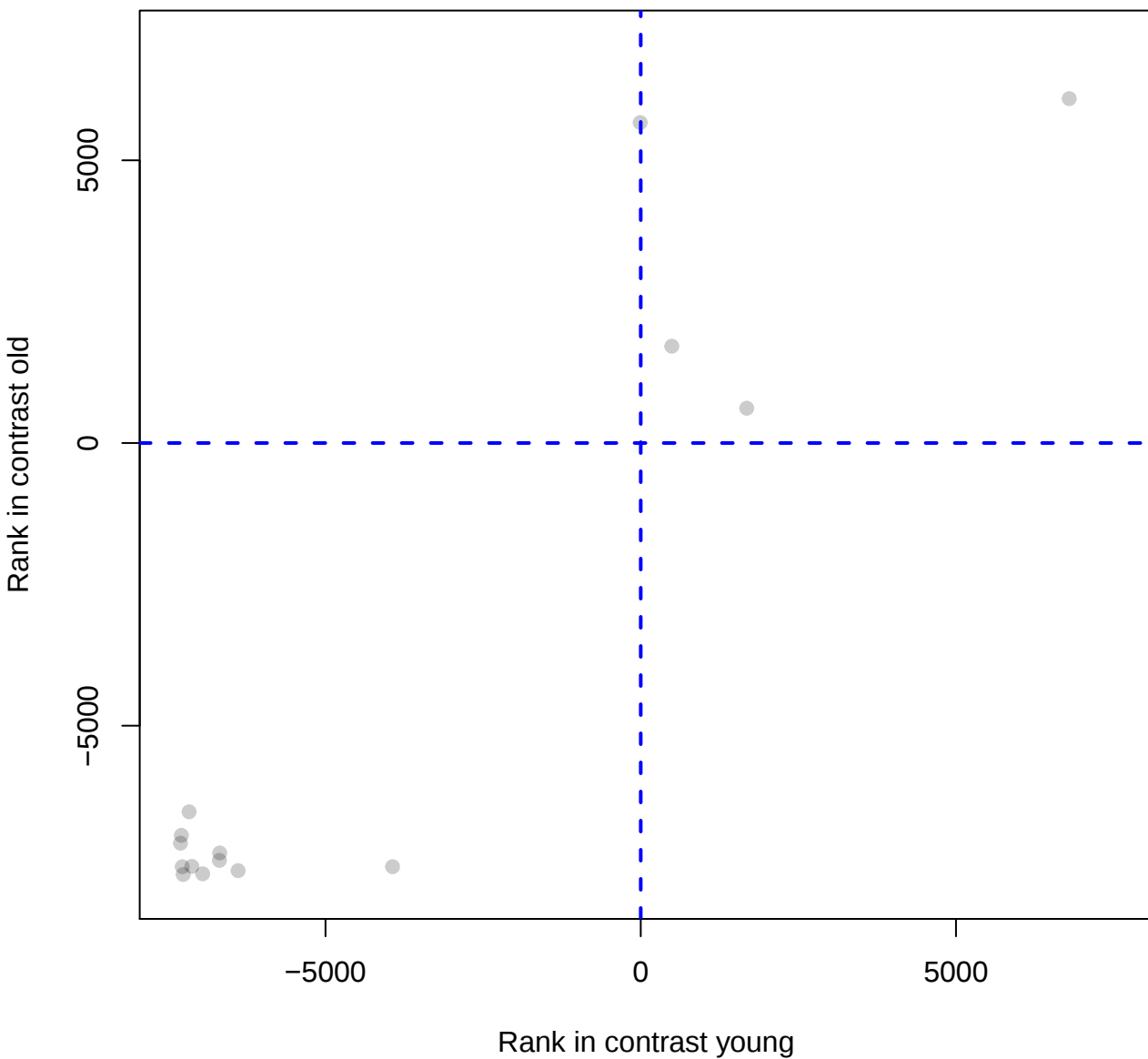
RELA_None_Macrophage_86665
