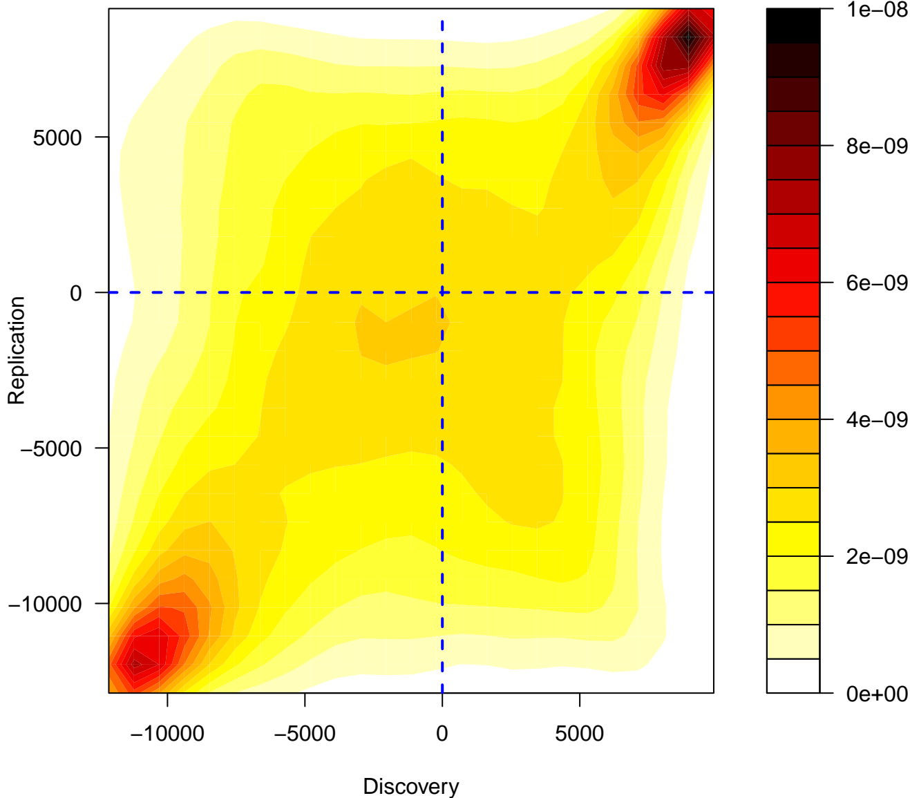
rank-rank plot
