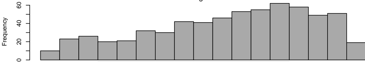
histogram
