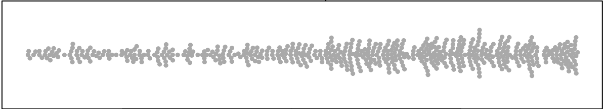
beeswarm plot
