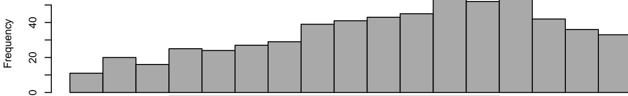
histogram
