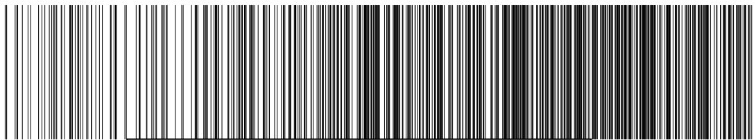
rugplot
