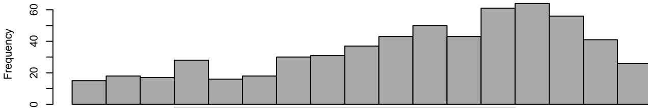
histogram
