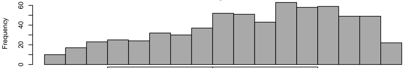
histogram
