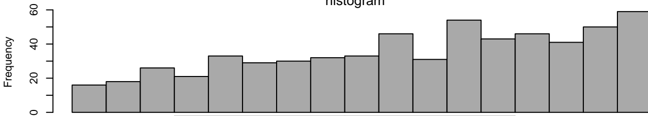
histogram
