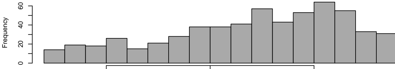
histogram
