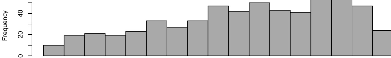
histogram
