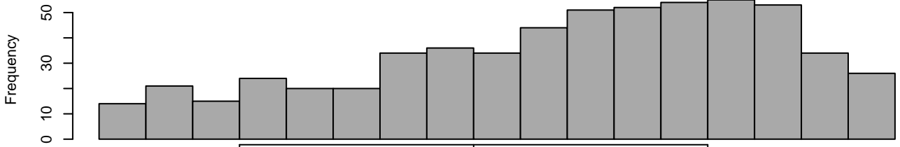
histogram
