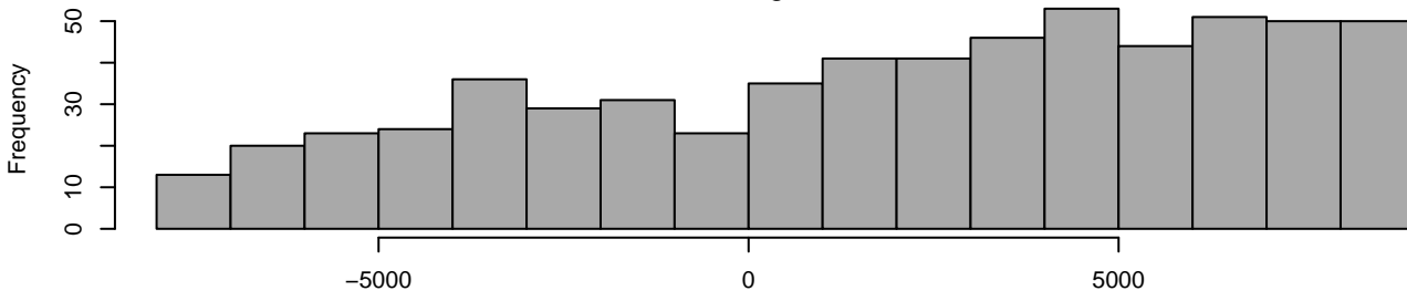
histogram
