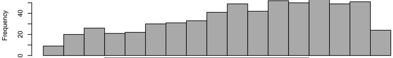
histogram
