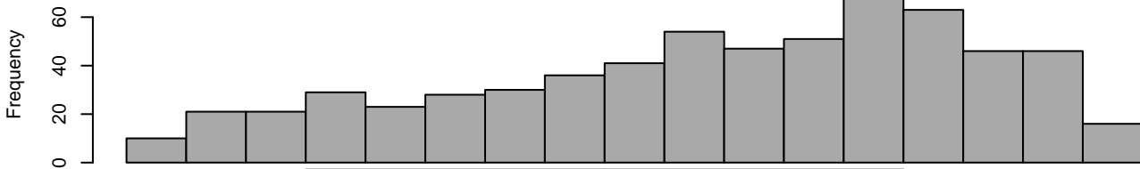
histogram
