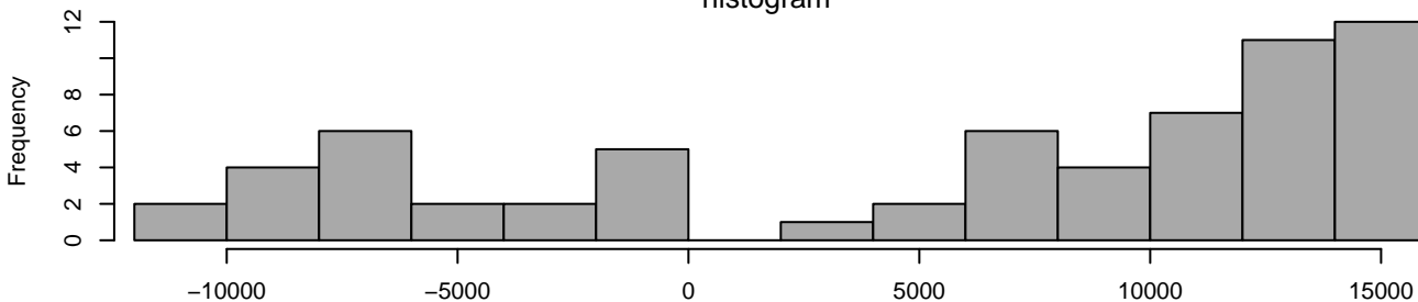
histogram
