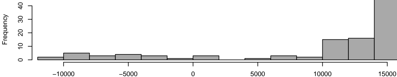
histogram
