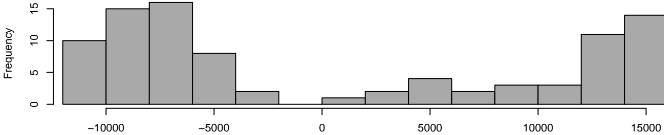
histogram
