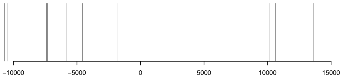
rugplot
